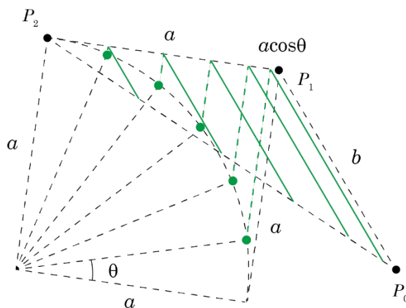
w -isoparametric lines
