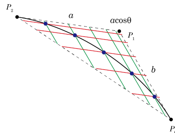
points on the curve
