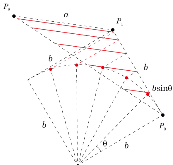
u -isoparametric lines
